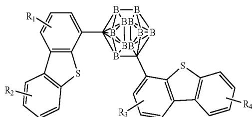
Compound 15G
