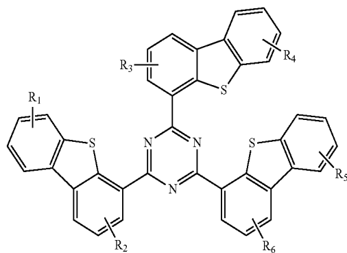
Compound 7G
