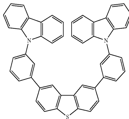
Compound 14
