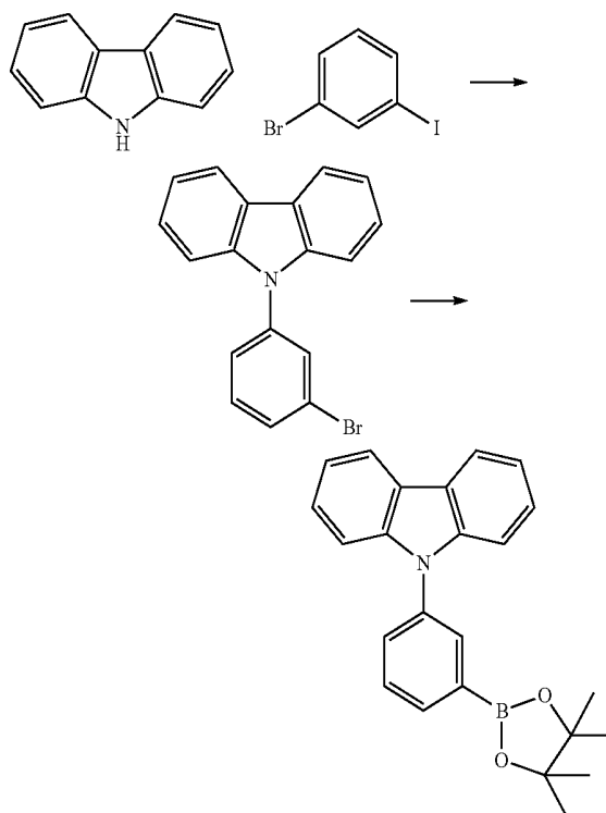
Compound 16
