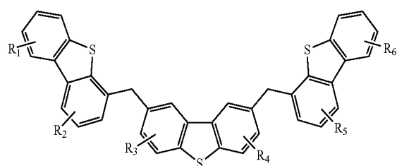
Compound 15G
