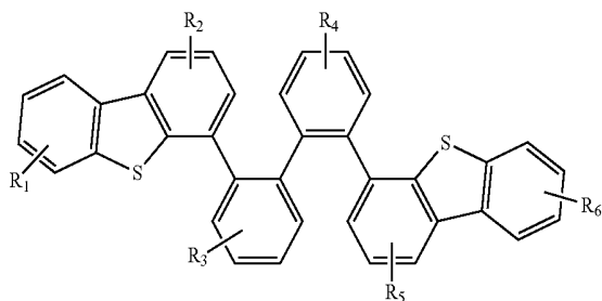
Compound 2G
