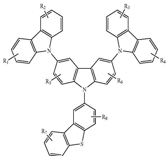
Compound 17G
