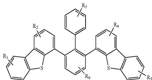
Compound 22G
