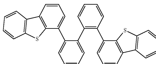
Compound 2
