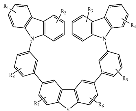
Compound 19G
