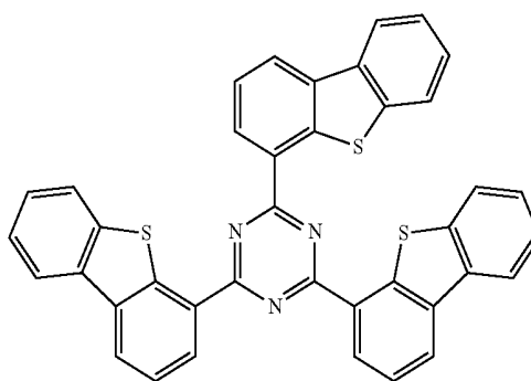
Compound 6
