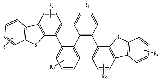
Compound 2G
