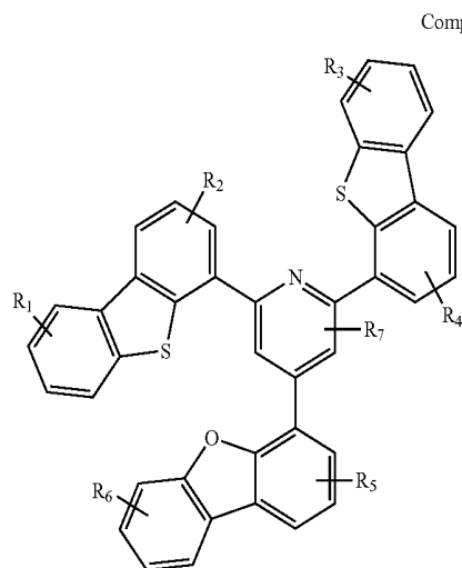
Compound 35G
