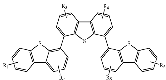
Compound 4G
