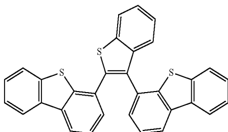
Compound 10
