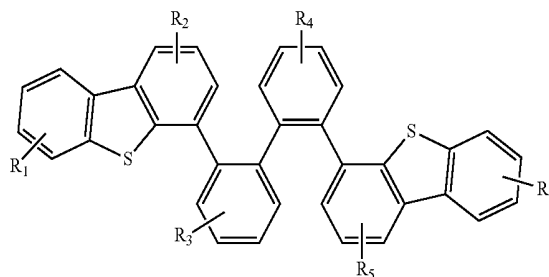
Compound 2G
