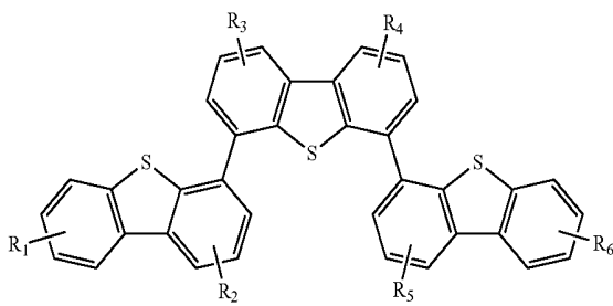
Compound 3G
