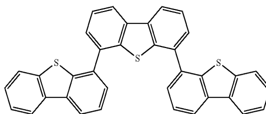
Compound 4
