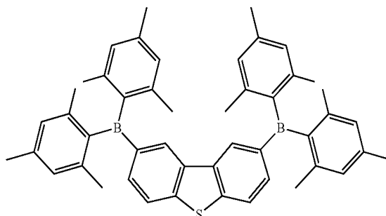
Compound 7
