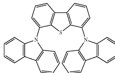
Compound 12G
