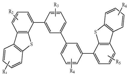
Compound 1G
