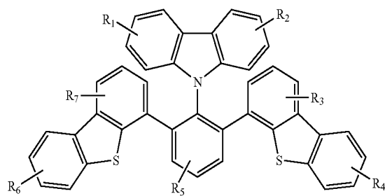
Compound 19G
