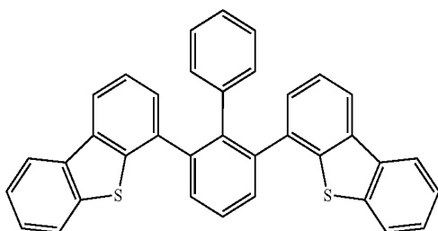
Compound 21
