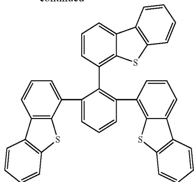
Compound 20
