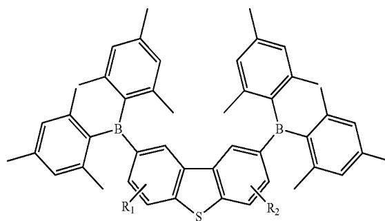
Compound 8G
