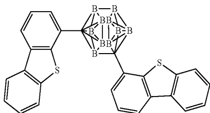
Compound 15
