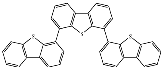
Compound 3
