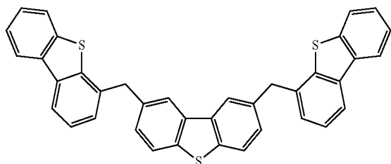
Compound 15
