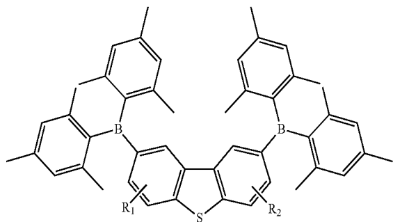
Compound 8G
