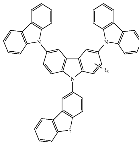
Compound 18
