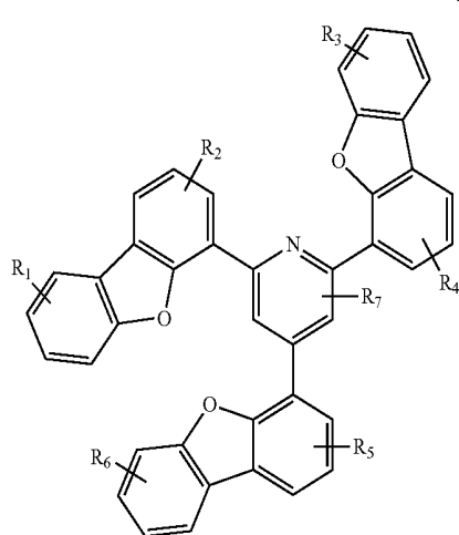
Compound 35G
