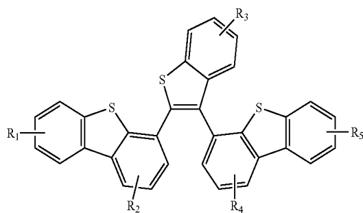
Compound 10G
