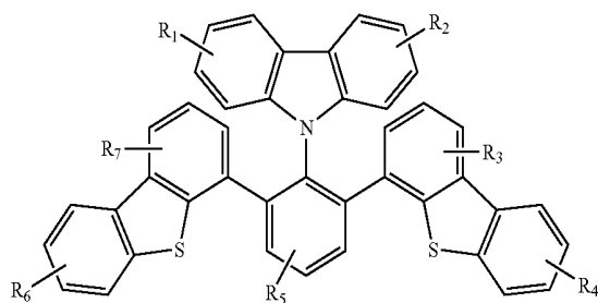
Compound 19G
