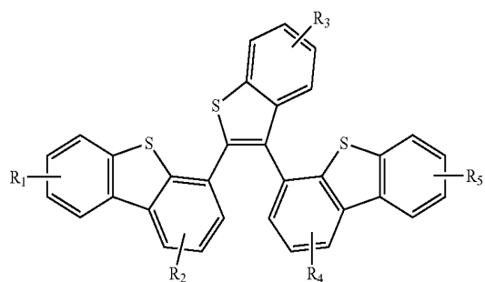
Compound 11G
