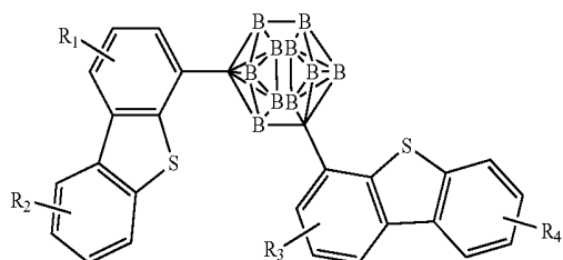
Compound 15G
