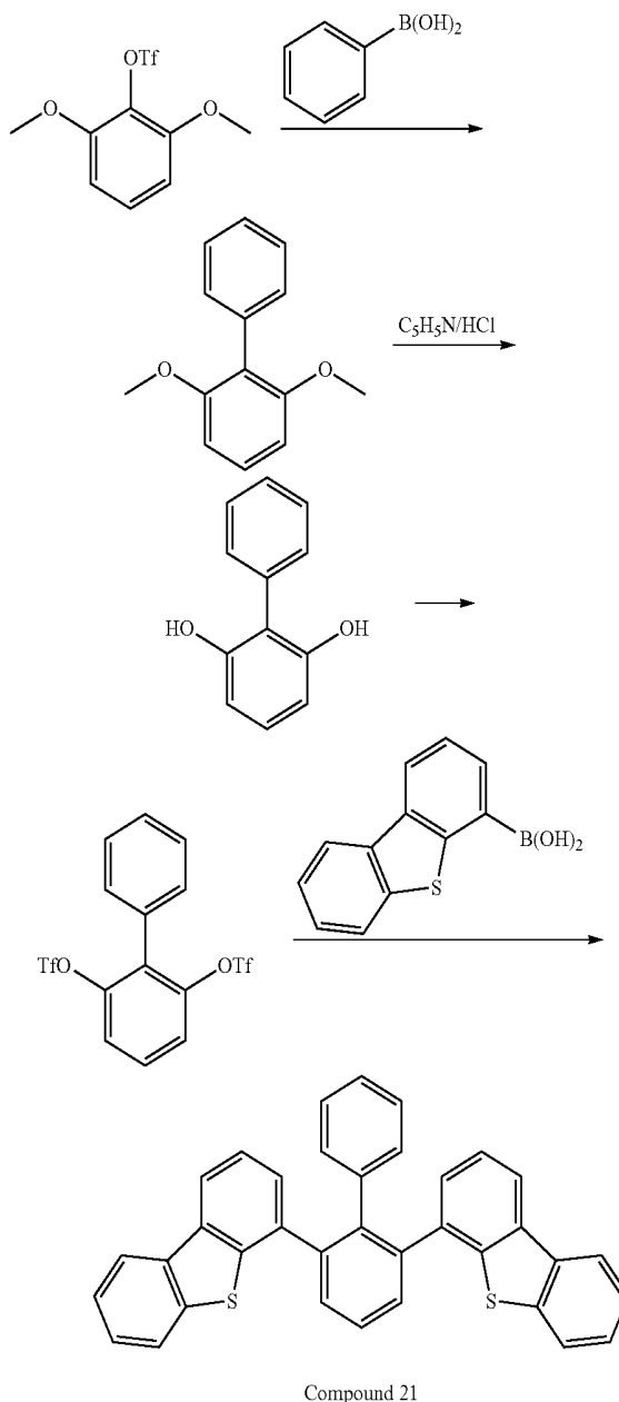
Compound 21
