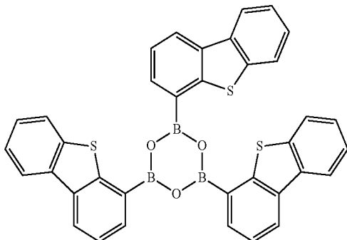
Compound 8
