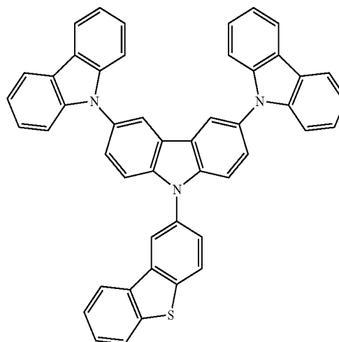
Compound 17
