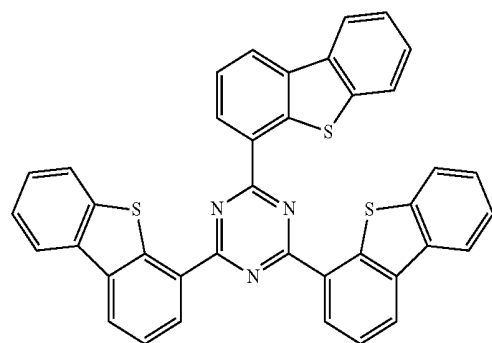
Compound 6
