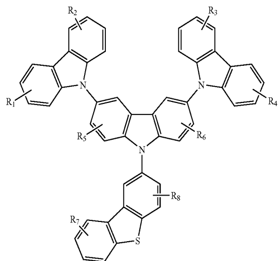
Compound 18G
