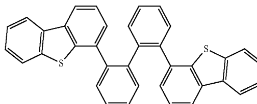
Compound 2
