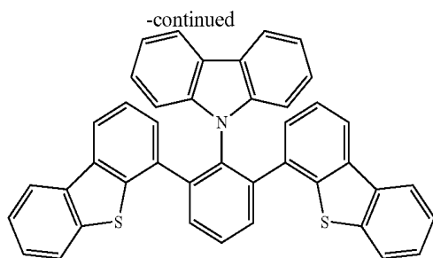
Compound 19
