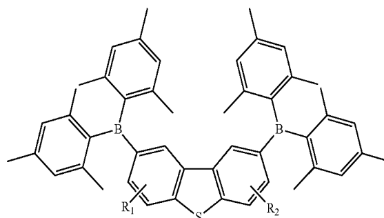
Compound 8G
